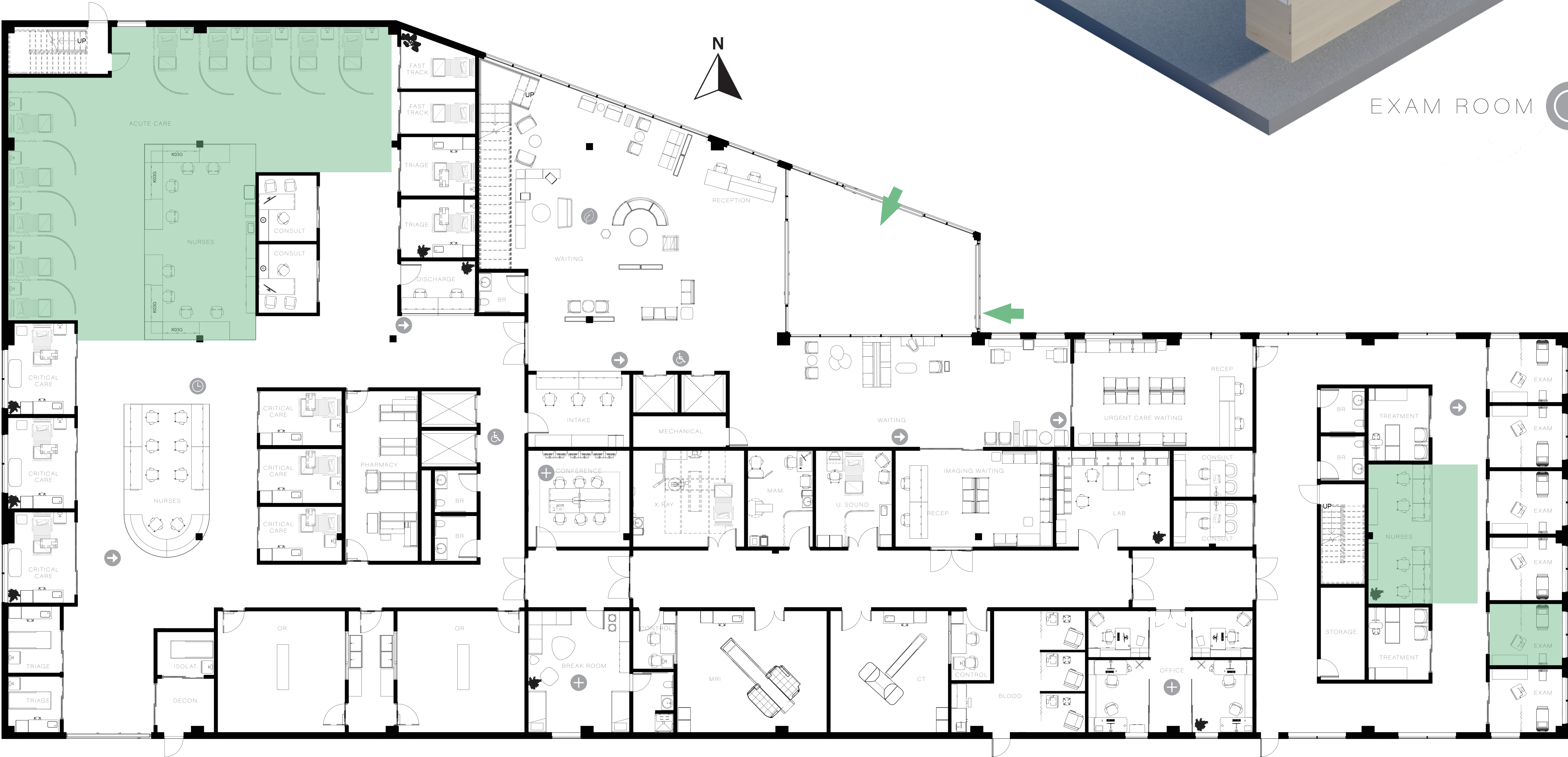
LEVEL ONE FLOOR PLAN 1/8"=1'
